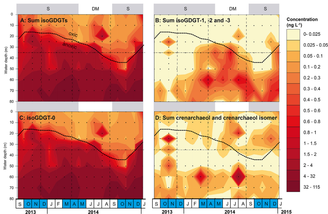
Fig. 3. Interpolated concentrations of isoGDGTs (in \text{ng L}^{-1} ) in SPM from Lake Chala sampled at approximately monthly intervals between September 2013 and January 2015. Concentrations of total isoGDGTs (A), sum of isoGDGTs-1, -2, and -3 (B), GDGT-0 (C), and sum of crenarchaeol and its isomer (D). The varying position of the oxic-anoxic boundary (oxycline, or depth to anoxia; van Bree et al., 2020), the static position of the sediment trap (thin dashed line at 35 m depth), and the SPM sampling grid (black dots) are indicated. Vertical dashed lines indicate the three months for which IPL GDGTs were also analyzed. The grey background shading shows the seasonal periods of upper water-column stratification (S) relative to those of deep mixing (DM), and blue shading in the calendar bars shows the typical timing of local rain seasons. (For interpretation of the references to color in this figure legend, the reader is referred to the Web version of this article.)
