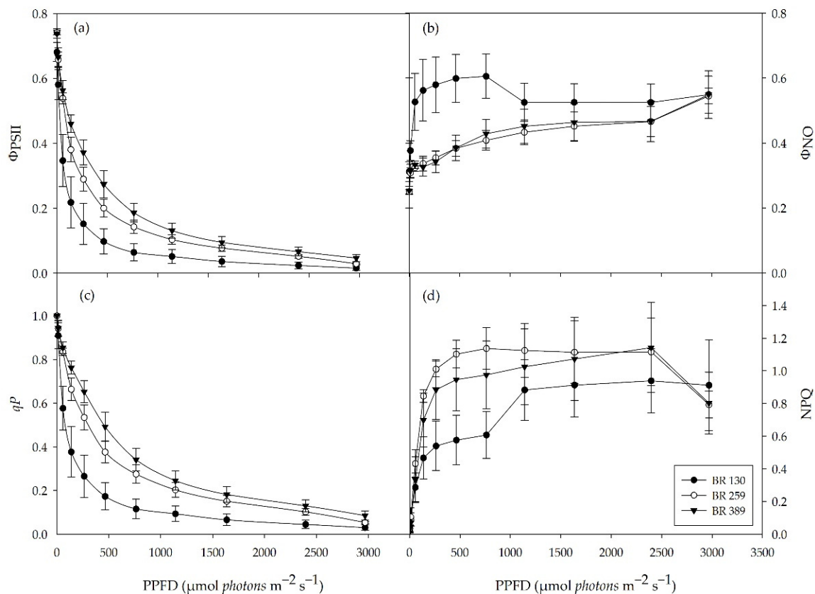
Figure 3. Chlorophyll a fluorescence light response curve. (a) Yield of \Phi_{PSII} and (b) yield of non-regulated quenching ( \Phi_{NO} ), (c) photochemical quenching ( qP ), and (d) non-photochemical quenching (NPQ) in Batavia lettuce cv ‘Blackhawk’ grown under three different light intensities (130, 259, 389 \mu\text{mol m}^{-2} \text{s}^{-1} ). Means value \pm standard error ( n = 5 , 30 DAT).
