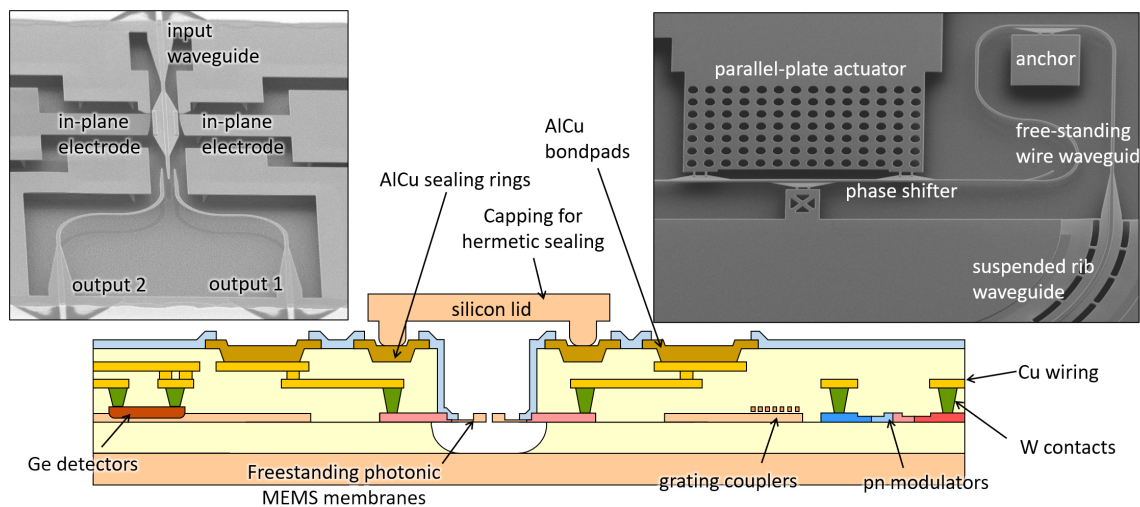
Fig. 1. MORPHIC silicon Photonic MEMS technology. Left: 1x2 switch [6], Right: Phase shifter. Bottom: cross section of the sealed silicon photonic MEMS platform [7].
