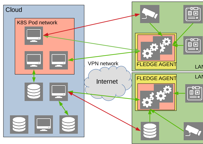
Fig. 3. Overview of network traffic flows in a cluster using FLEDGE nodes. Green arrows indicate possible traffic flows.
