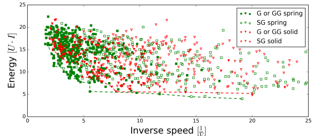
Fig. 2: Summary of all the parameter configurations that led to acceptable gaits for both, stiff and compliant leg configurations.
