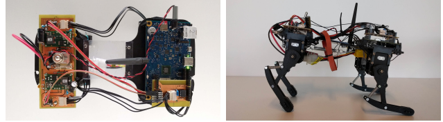
Fig. 1: Top down view and side view of Tigrillo.
