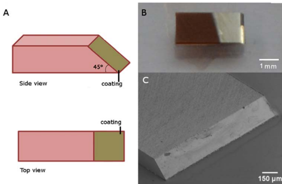
Fig. 2. Master mold with polished tilted micromirrors fabricated in polyimide. (A) Schematic top and side view of the polished polymer plug. (B) A simple master mold is created by gluing two of those polymer plugs, coated with aluminum (or gold), to a microscope slide. The sample can be placed in between the polymer plugs. (C) SEM micrograph of the polished polymer tilted mirror.
