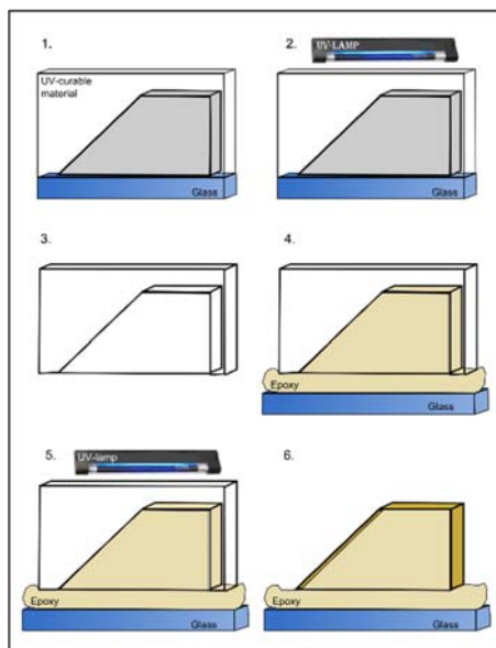
Fig. 10. Schematic overview of the replication process.
