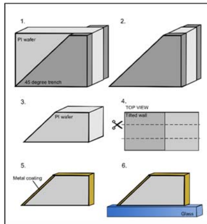
Fig. 9. Fabrication procedure of the polymer-based master mold.
