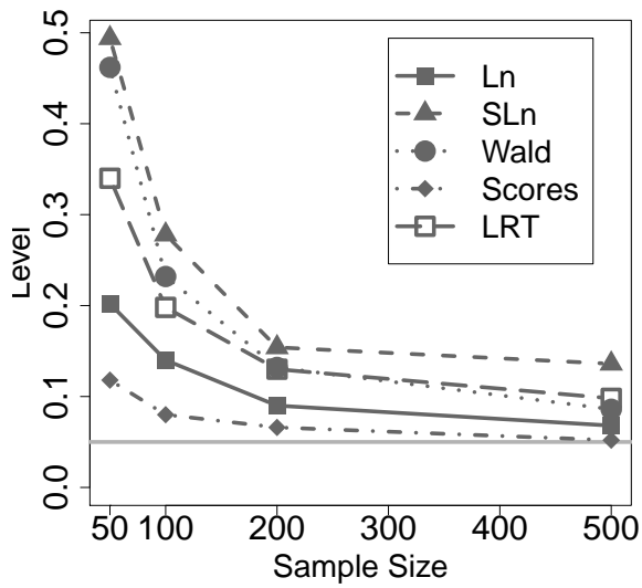
(a) Asymptotic approximation
