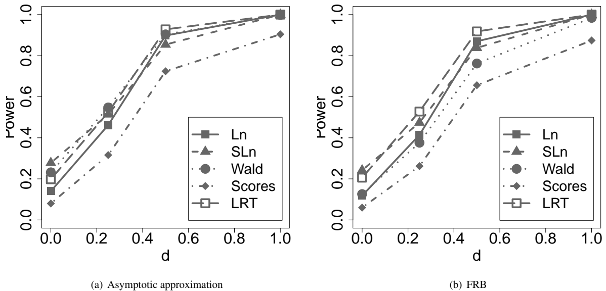
Figure 8: Empirical power for samples with 10% of high-leverage outliers. Empirical power levels for contaminated samples of size n = 100 as a function of the parameter d in (26). The left and right panels contain the results obtained with the asymptotic \chi^2 approximation and with the FRB, respectively.
