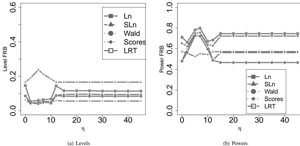
Figure 5: Empirical levels and powers (for d = 0.25 ) for different outlier configurations, for samples of size n = 200 .
