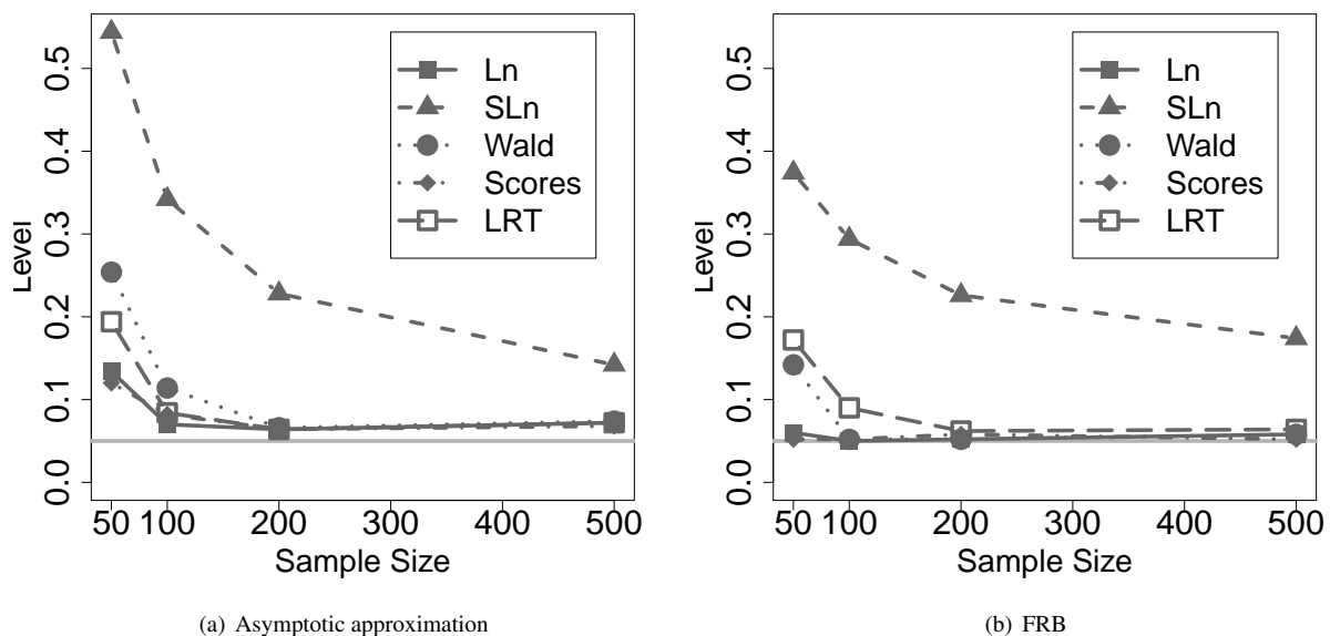
Figure 2: Accuracy of level. Empirical levels as a function of the sample size, when no contamination is present. The left panel contains the results obtained by using the asymptotic \chi^2 approximation. Estimating the p -values using FRB yields the empirical levels displayed in the right panel.
