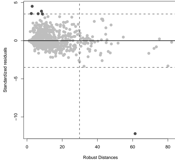
Figure 9: Plot of standardized residuals versus robust Mahalanobis distances for the linguistic data. The horizontal dashed lines indicate \pm 3.5 standard deviations. The vertical line corresponds to the 99.5% quantile of a \chi_{13}^2 distribution. Observations that are beyond this line can be considered high-leverage points.
