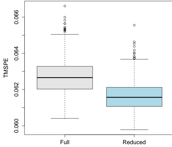
Figure 10: Boxplots of 500 replicates of 5-fold cross-validation estimates of the trimmed mean squared prediction error (10% trimming proportion) for the full and reduced models.
