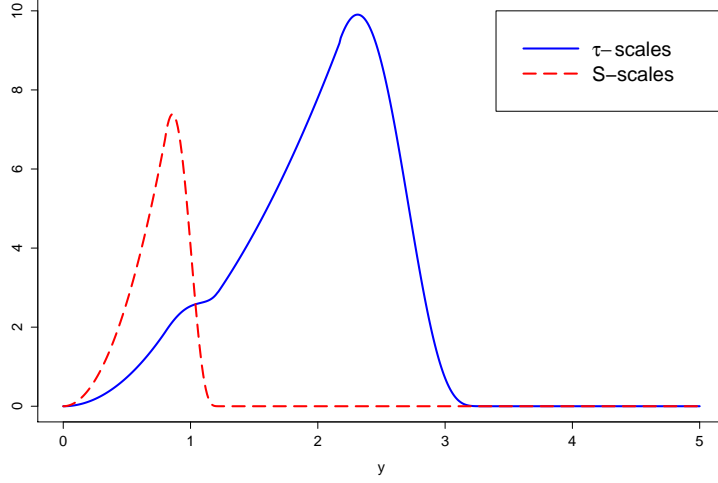
Figure 1: Response part of the standardized second-order influence function of the robust test statistic for a normal error distribution.
