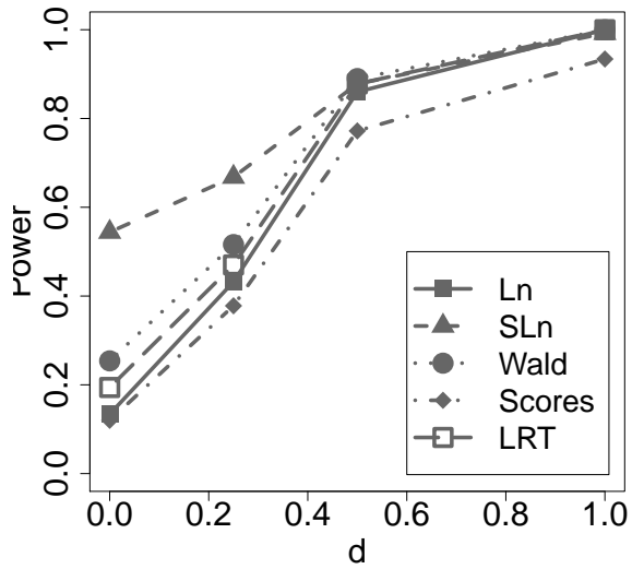
(a) Asymptotic approximation
