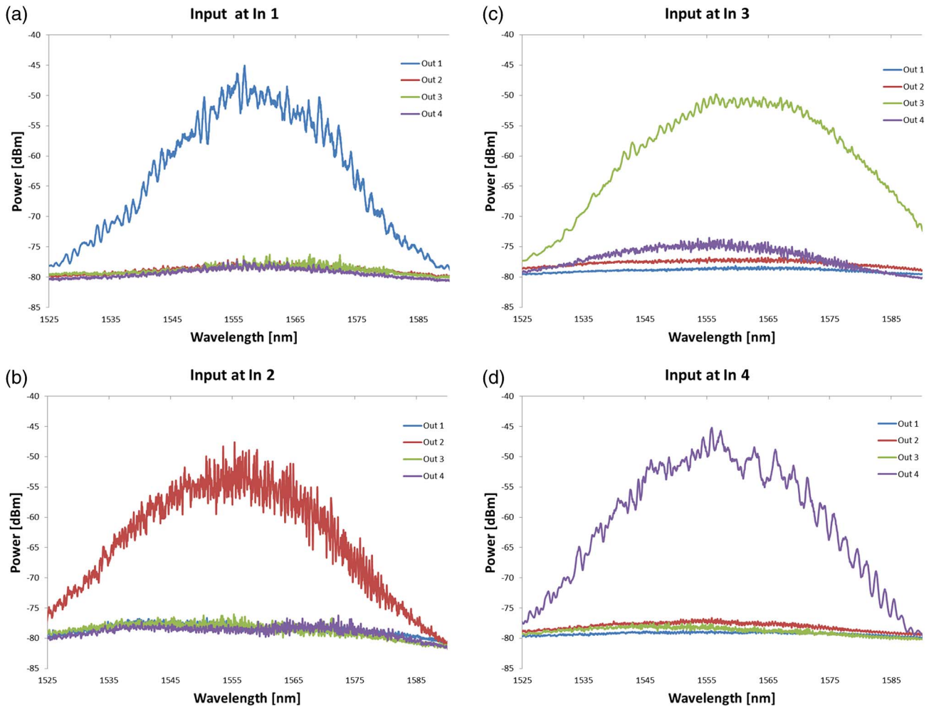
Fig. 5. Transmission spectrum for input at (a) In 1, (b) In 2, (c) In 3, and (d) In 4. The measurement was done using an IR camera to read monitors M1 to M4 simultaneously.
