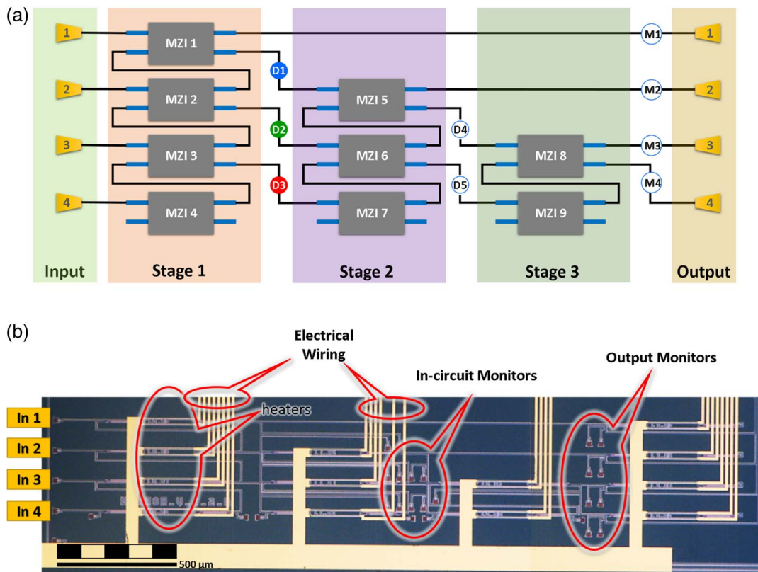
Fig. 2. (a) Schematic of the integrated implementation of the circuit using MZIs. The optical input and the output are done using grating couplers. Detectors D1 to D5 are implemented using optical taps connected to a grating coupler, for monitoring using an IR camera. The same approach was used with output monitors M1 to M4, which are used to monitor the optical power at the output of the circuit. (b) Microscope image of the fabricated device.
