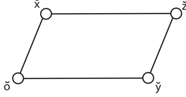
Figure 1: Parallelogram \check{o}\check{y}\check{z}\check{x}\check{o} representing the equation [z] = [\kappa][x][y] in \mathbb{Z}^7 .
