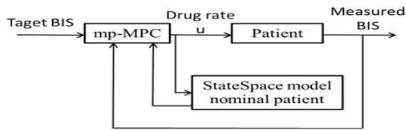
Fig. 6. Case 2: mp-MPC without nonlinearity compensation - control scheme
