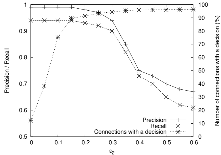
Figure 8. Impact of the \epsilon_2 parameter in terms of the precision and recall, characterizing the accuracy of the detection algorithm, and the number of connections with a decision, characterizing the connections that are not labeled as 'unknown'.
