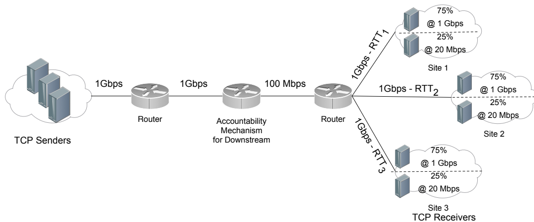
Figure 2. Used network topology for all experiments with a central bottleneck of 100 Mbps. The topology consists of 3 sites, with various RTTs, that request content from a single TCP sender site. 25% of all TCP receivers experience an additional bottleneck of 20 Mbps.
