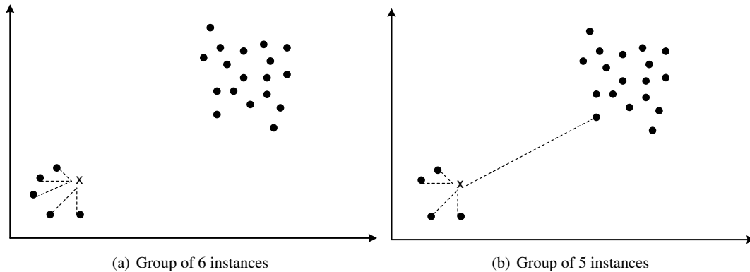
Figure 6. Graphical overview of an illustrative 2-dimensional outlier calculation for a group of 6 instances (a) and 5 instances (b). As k is set to 5, only the group of 5 instances are identified as outliers.
