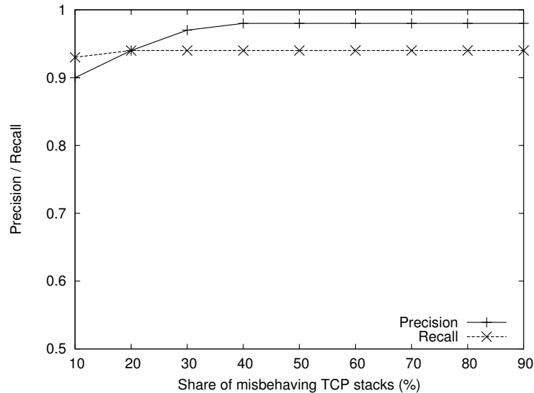
Figure 9. Precision and recall for an increasing share of misbehaving TCP stacks.
