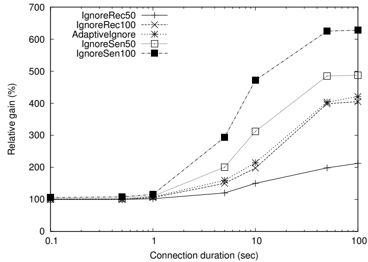
Figure 4. Relative gain of misbehaving TCP stacks given an increasing connection duration.
