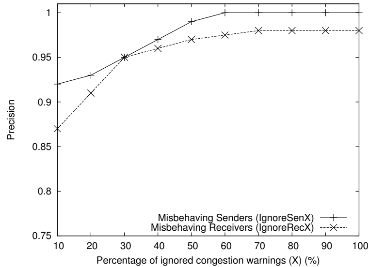
Figure 10. Precision and recall for an increasing level of misbehaving in TCP stacks.
