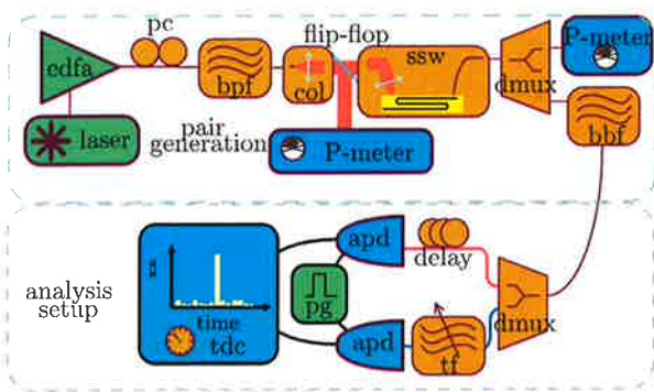
Fig. 1. (Color online) Experimental setup. Photon flux is generated in the top part of the setup and the bottom part is used to analyze this flux in the Stokes and anti-Stokes bands. Laser, CW laser source at 1539.8 nm; EDFA, erbium-doped fiber amplifier; pc, polarization controller; bpf, bandpass filter to clean the pump beam; col, collimation lens; P-meter, power meter; flip flop, mirror used to measure the input power; SWW, silicon wire waveguide; demux, demultiplexer; bbf, bandblock filter; tf, tunable filter; apd, avalanche photodiode; pg, pulse generator; tdc, time-to-digital converter + computer.
