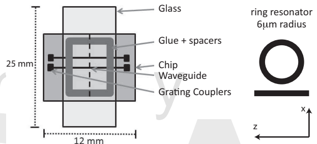
Fig. 3. Schematic top view of a device consisting of a SOI substrate with LC cladding, sealed off by a glass-plate with a transparent ITO electrode and polyimide alignment layer (left). Schematic top view of a single ring resonator with the straight waveguide below (right).
