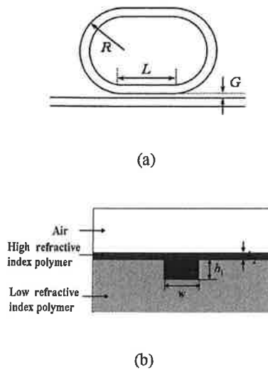
Fig. 1 (a) Schematic of microring resonator and (b) cross section of polymer waveguide.
